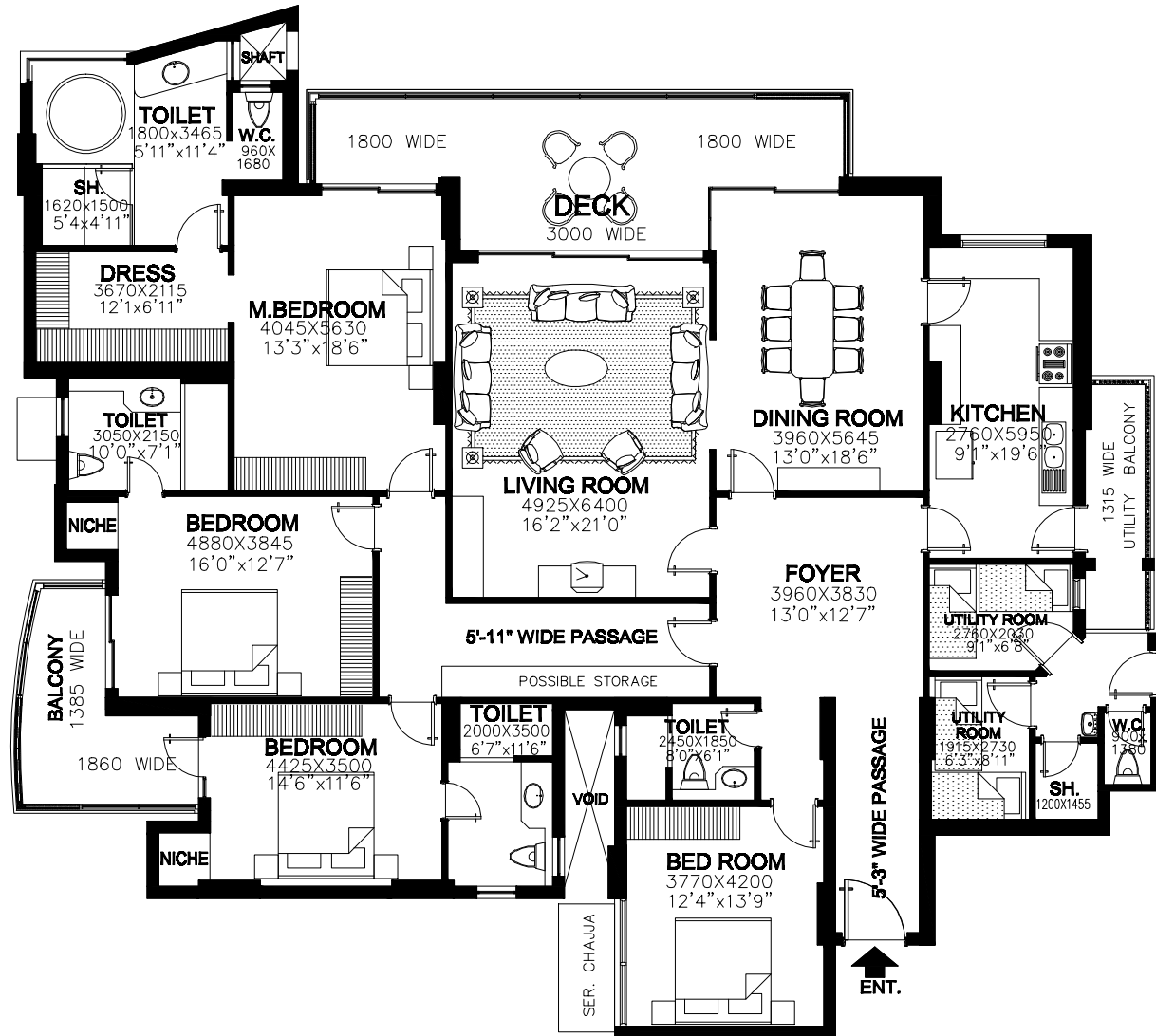
TENTATIVE PLAN OF APARTMENT NO. 1
